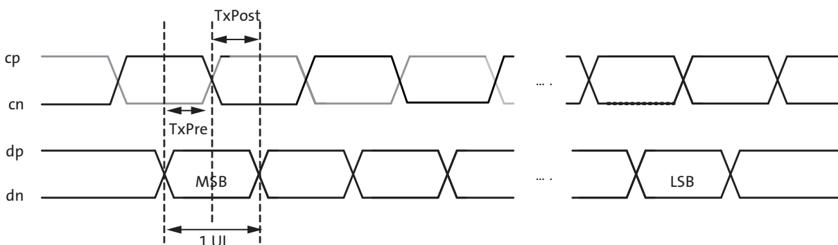
Figure 12: Timing Diagram
